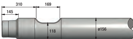
FIGURE 292 NPK H-20X / E
