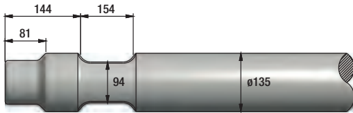
FIGURE 234 MSB SAGA 200II / 220
