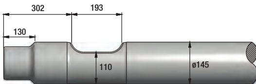
FIGURE 291 NPK H-16X / E
