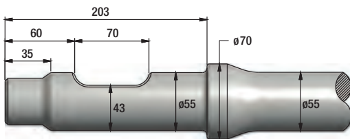
FIGURE 162 KRUPP HM85 / 90 / 90V
