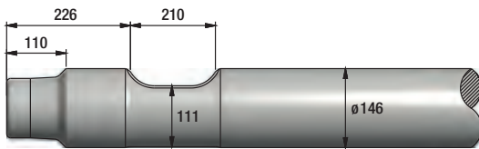
FIGURE 274 NPK E-18X / E-218
