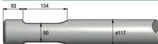
FIGURE 386 SOCOMEK MDO 900V
