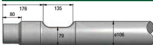
FIGURE 261 NPK E-207 / GH6
