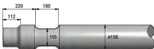
MONTABERT (BLUE LINE) XL2600
