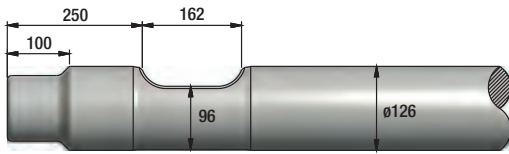
FIGURE 289 NPK H-10XB / H-10XE
